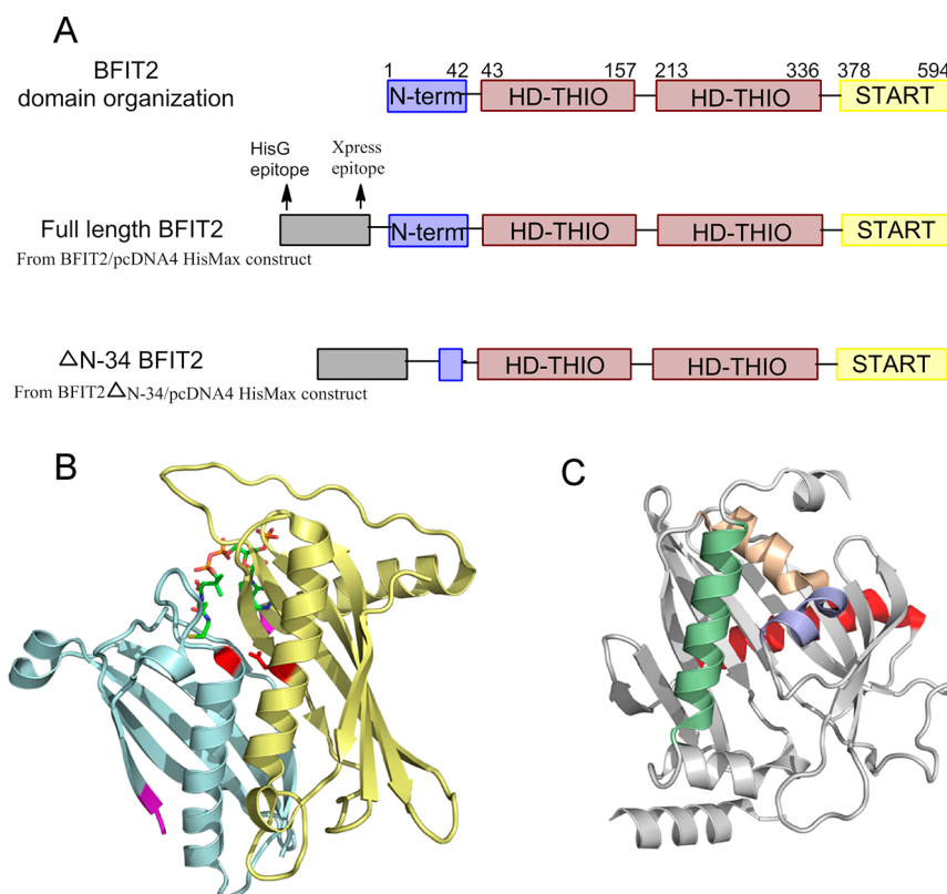
Figure 1. (A) Diagram of the domain organization in human BFIT2 and the two human BFIT2 gene constructs that were used in this work. N-term corresponds to the MLS, HD-THIO to the hotdog-fold domain, and START to the StarD14 domain. (B) One subunit of the trimeric human CACH (ACOT12) double hotdog-fold unit (PDB entry 3B7K). The first hotdog-fold domain is colored pale yellow and the second hotdog domain pale cyan. Residues 151–180, which form the domain–domain linker, are disordered and are therefore not shown in the structure. Residues 150 and 181 are colored magenta. A CoA ligand, bound to one of the two active sites, is shown as sticks with carbon atoms colored green, nitrogen atoms blue, oxygen atoms red, and the sulfur atom yellow. The posited catalytic residues Gly202 and Asp36 are colored red. (C) BFIT2 START domain StarD14 (PDB entry 3FO5). The conserved \alpha -helices are colored. Gatekeeper helix \alpha 4 is colored pale green.
