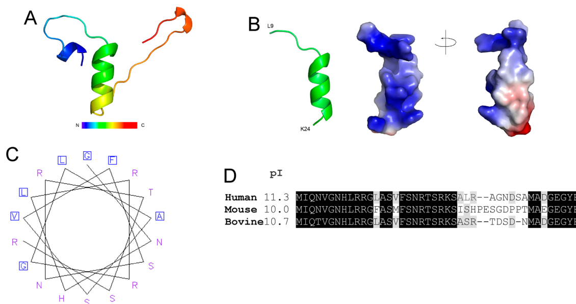
Figure 3. (A) Predicted tertiary structure of the hBFIT2 N-terminal region (residues 1–42). (B) Electrostatic vacuum surface of the central \alpha -helix (hBFIT2 residues 9–24). (C) EMBOSS pepwheel diagram of hBFIT2 residues 5–24. (D) Sequence alignment and estimated pI value of the N-terminal regions of BFIT2 from various mammalian species.
