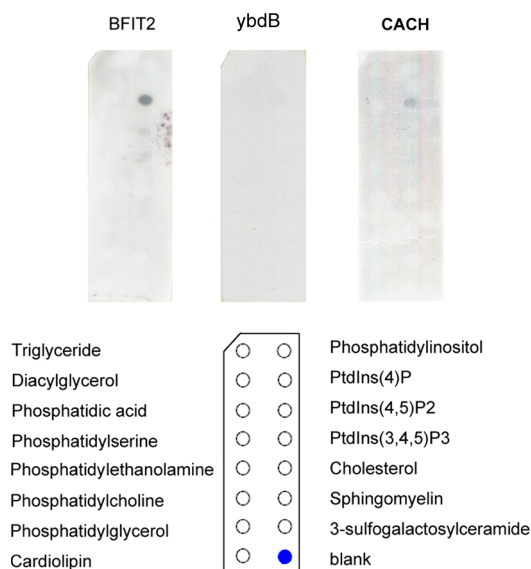
Figure 9. Protein–lipid overlay assays in which Membrane Lipid Strips (Echelon Bioscience Inc.) were separately treated with 0.5 \mu\text{g/mL} hBFIT2 (purified as described above), 0.1 \mu\text{g/mL} hCACH, or 6 \mu\text{g/mL} HisG and Xpress-tagged ybdB in PBS-T and then imaged. See Materials and Methods. The lipid positions are identified in the key.
