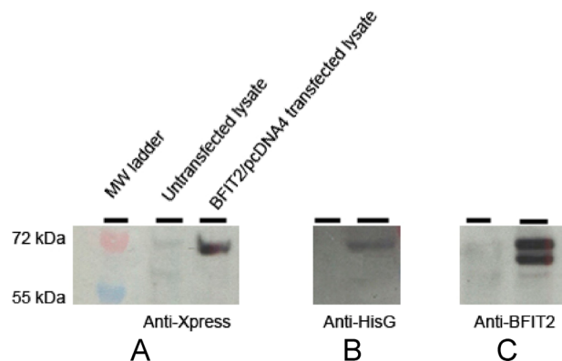
Figure 2. Immunoblot of untransfected (middle or left lane) and hBFIT2/pcDNA4 -transfected HEK293T/17 cell lysates (right lane) using anti-Xpress antibody (A), anti-HisG antibody (B), and anti-BFIT2 antibody (C).
