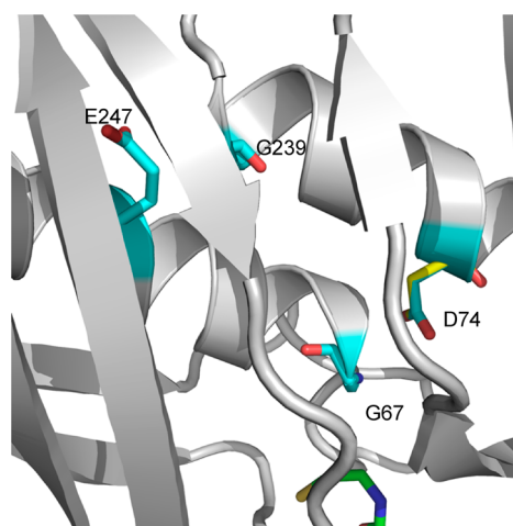
Figure 7. Snapshot of the two active sites of the double hotdog-fold unit of hBFIT2 modeled in PHYRE2 using the double hotdog-fold unit of CACH (ACOT12) (PDB entry 3B7K), which shares 60% sequence identity, as the template. The thiol end of the superimposed CACH CoA ligand is shown at the bottom of the figure as sticks using the same coloring pattern used in Figure 1B. The putative hBFIT2 catalytic residues are shown as sticks with carbon atoms colored cyan, oxygen atoms red, and nitrogen atoms blue. The corresponding residues of the superimposed CACH (carbon atoms colored yellow) are coincident.
