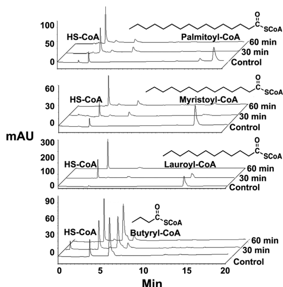
Figure 8. Reversed-phase HPLC chromatograms of reaction mixtures initially containing 0.34 \mu\text{M} purified recombinant hBFIT2 and 50 \mu\text{M} fatty acyl-CoA substrate in 50 \text{ mM} HEPES buffer ( \text{pH } 7.5 , 37^\circ\text{C} ). Aliquots were removed at 30 and 60 min incubation periods for analysis. The control reaction mixtures, which lacked hBFIT2, were incubated for 2 h. See Materials and Methods for details.
