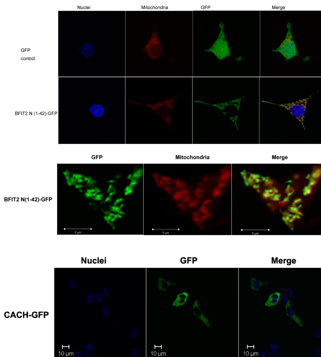
Figure 4. Confocal imaging of the GFP and the BFIT2 N(1–42)–GFP fusion protein in transfected HEK 293T/17 cells (top). Close-up of the fluorescence from the BFIT2 N(1–42)–GFP fusion protein and the mitochondria dyed with Mitotracker CMXRos (middle). Confocal imaging of the CACH–GFP fusion protein showing distributive localization in the transfected HEK 293T/17 cells (bottom). The nuclei were stained with Hoechst 33342.
